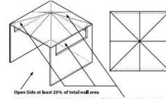
Open Side at least 25% of total wall area 30% or more in total of the remaining wall area is open and unrestricted Outdoor Area - Example 4
